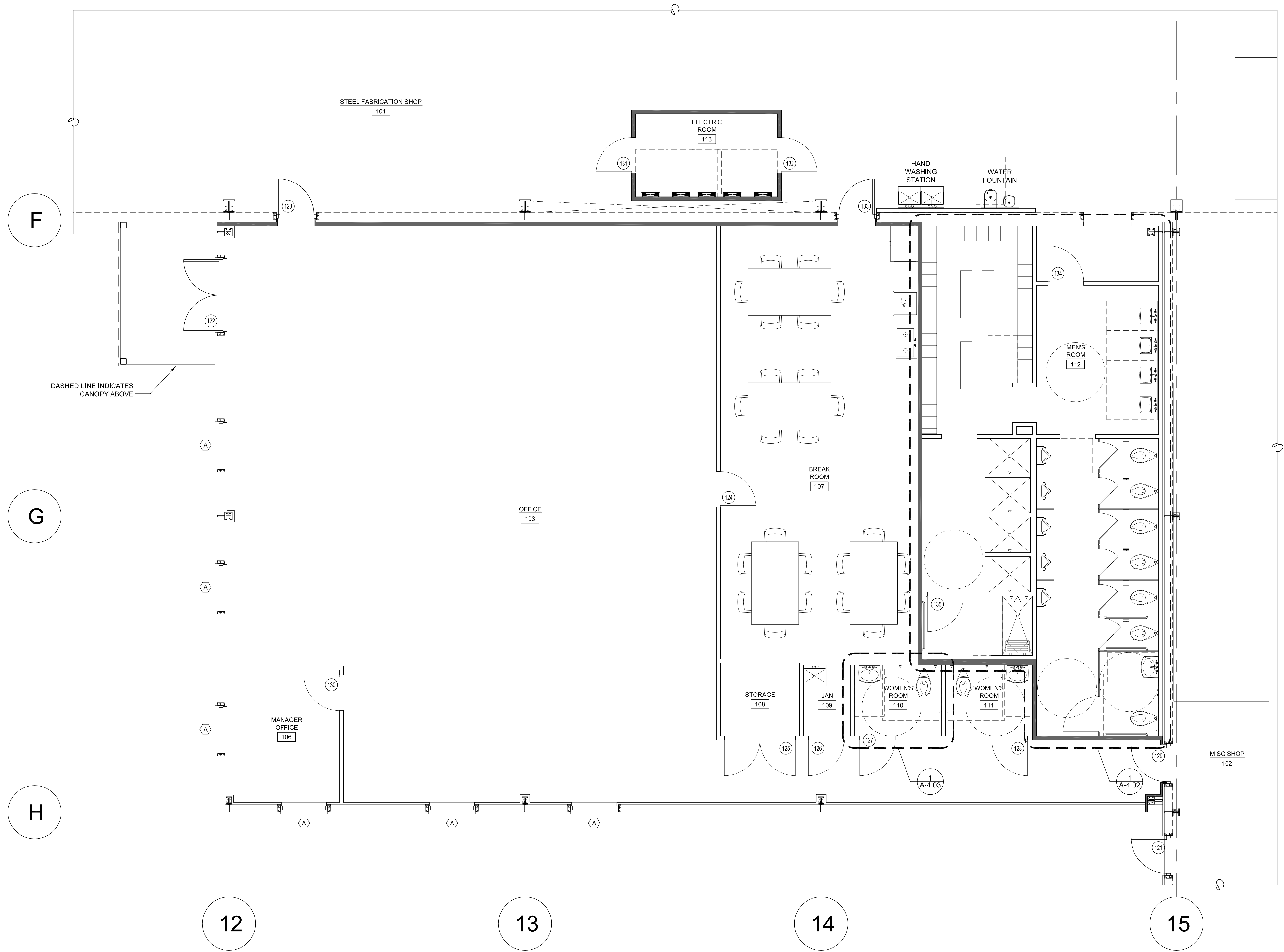
ENLARGED PLAN @ OFFICE SCALE: 1/4" = 1'-0"
